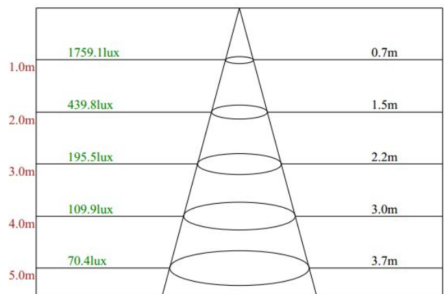
Beam angle of C0plane40.70
